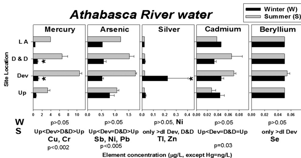
Fig. 3. Element concentrations (mean \pm SE, expressed in \mu\text{g/L} , except for Hg, which is expressed in ng/L) in water from the AR collected in winter (W, black bars) and summer (S, gray bars). Up, AR upstream ( n = 3 ); Dev, AR downstream/near development ( n = 7 ); D&D, AR downstream and Athabasca Delta ( n = 6 ); LA, Lake Athabasca ( n = 1 ); dl, detection limit and only > dl Dev, greater than dl only at sites near development. *Increases near development and downstream that were not statistically significant (power \beta < 0.171 ). The distribution of elements listed below panels is similar to that in the panel above, and statistics refer to all elements with similar distributions.
